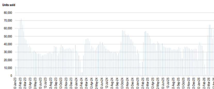
Figure 1: Iceberg 20-city real-time secondary weekly sales data
